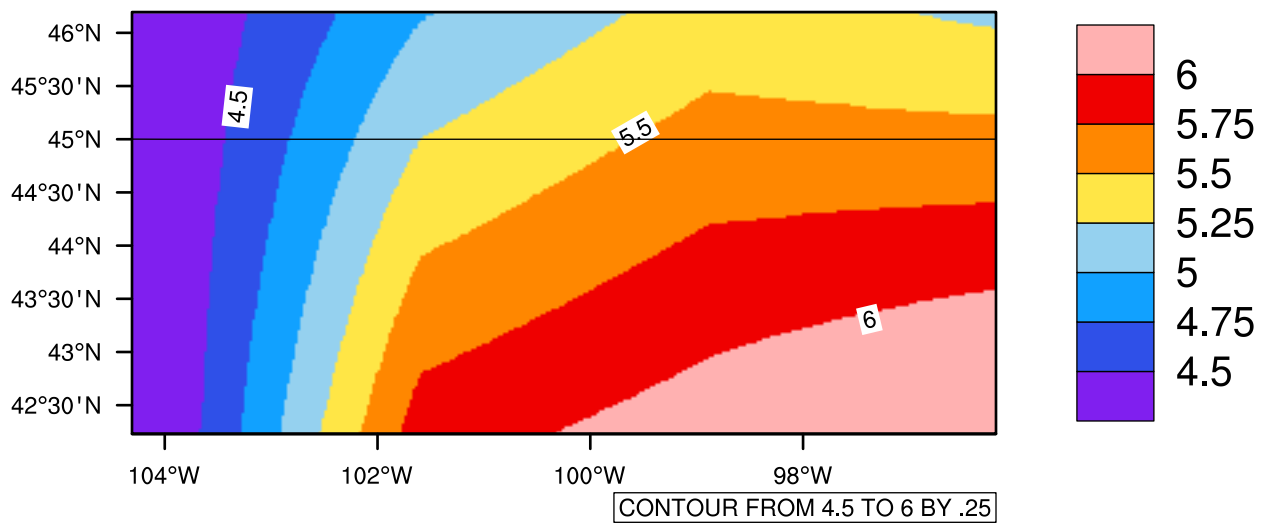
Yearly tasmin(c) In 2090-2099 GFDL-ESM2M RCP45 - South Dakota
