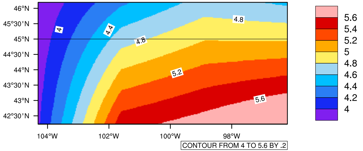
Yearly tasmin(c) In 2040-2049 GFDL-ESM2M RCP85 - South Dakota
