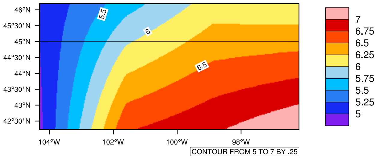
Yearly tasmin(c) In 2050-2059 GFDL-ESM2M RCP85 - South Dakota
