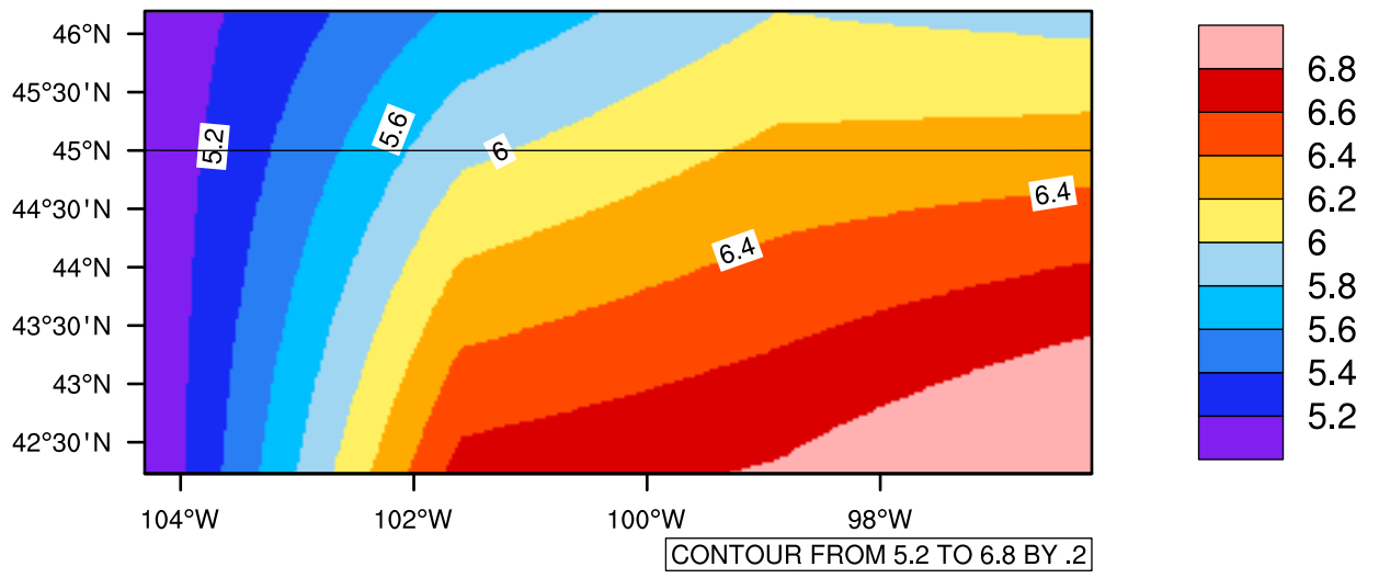
Yearly tasmin(c) In 2060-2069 GFDL-ESM2M RCP85 - South Dakota
