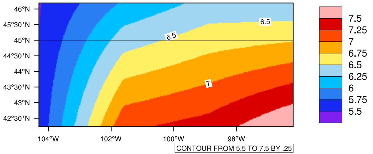
Yearly tasmin(c) In 2070-2079 GFDL-ESM2M RCP85 - South Dakota
