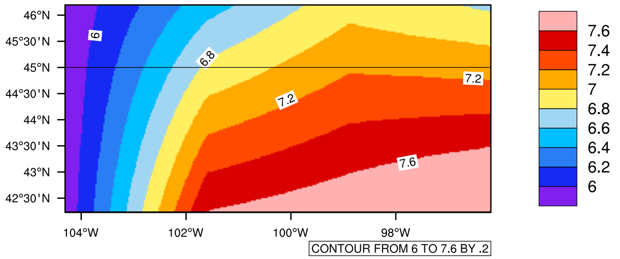
Yearly tasmin(c) In 2080-2089 GFDL-ESM2M RCP85 - South Dakota
