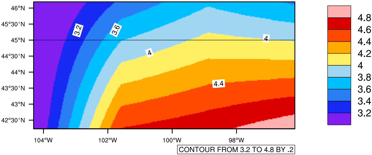
Yearly tasmin(c) In 1975-2005 GFDL-ESM2M historical - South Dakota
