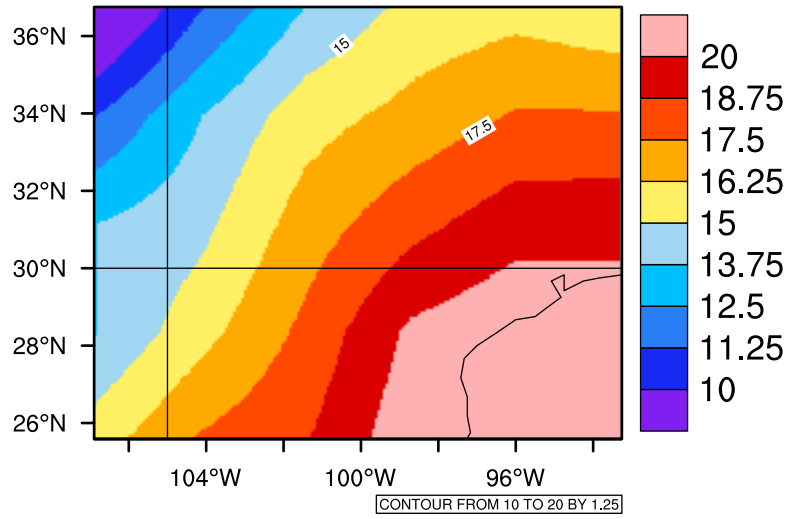
Yearly tas(c) In 2030-2039 GFDL-ESM2M RCP45 - Texas
