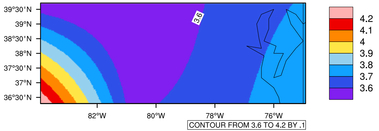
Yearly pr (mm/day) In 2050-2059 GFDL-ESM2M RCP85 - Virginia
