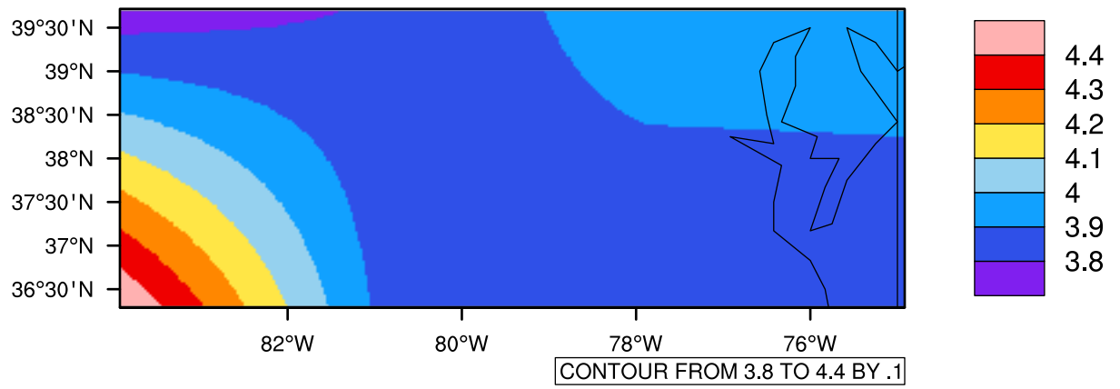
Yearly pr (mm/day) In 2080-2089 GFDL-ESM2M RCP85 - Virginia
