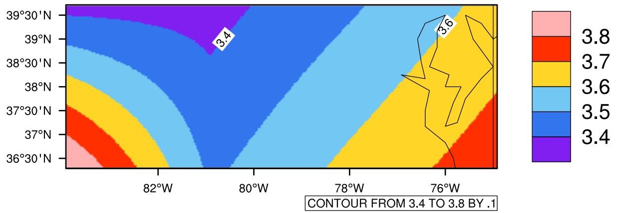
Yearly pr (mm/day) In 2090-2099 GFDL-ESM2M RCP85 - Virginia
