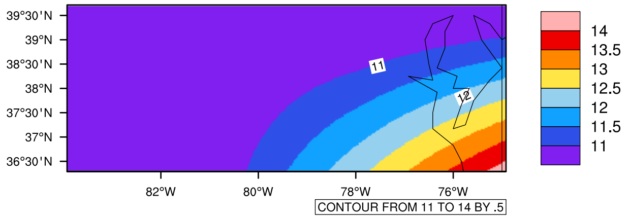
Yearly tas(c) In 2020-2029 GFDL-ESM2M RCP45 - Virginia
