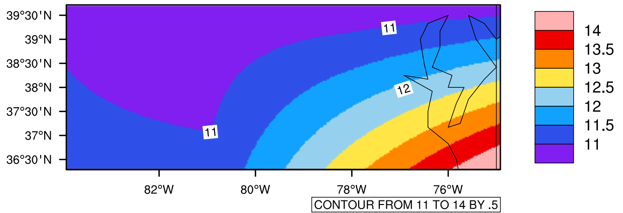
Yearly tas(c) In 2030-2039 GFDL-ESM2M RCP45 - Virginia
