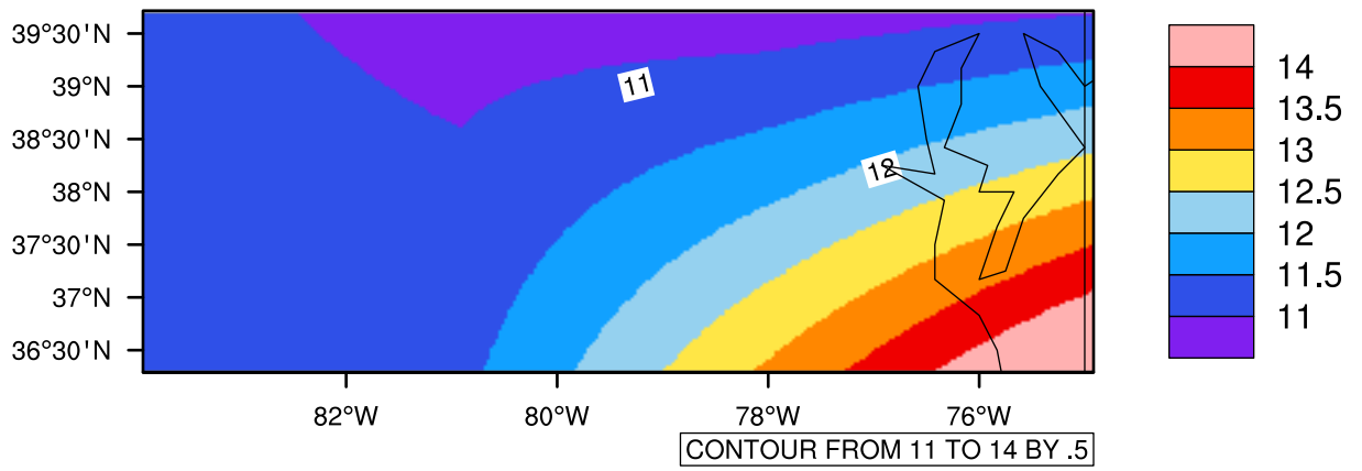
Yearly tas(c) In 2040-2049 GFDL-ESM2M RCP45 - Virginia
