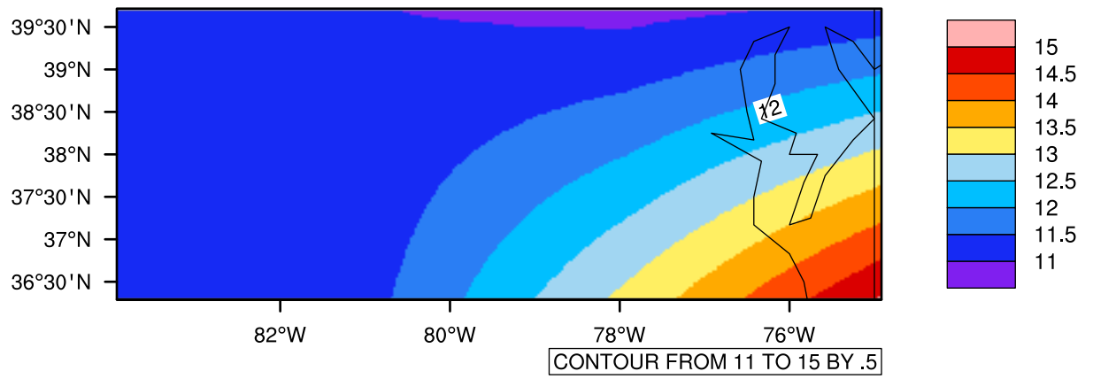
Yearly tas(c) In 2050-2059 GFDL-ESM2M RCP45 - Virginia
