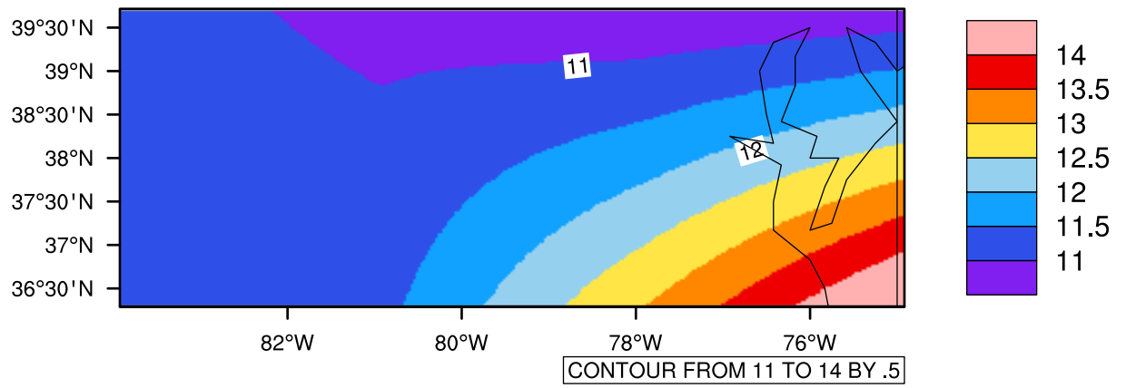
Yearly tas(c) In 2060-2069 GFDL-ESM2M RCP45 - Virginia
