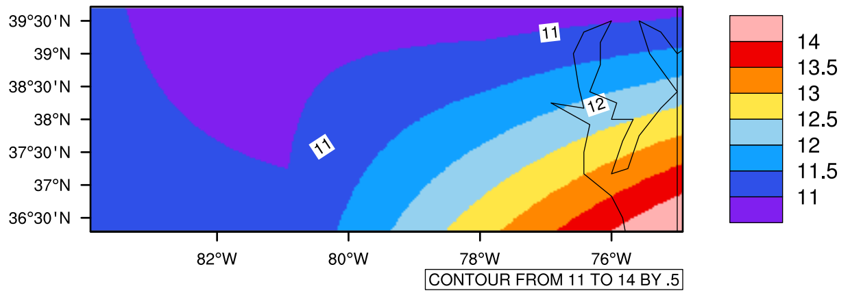
Yearly tas(c) In 2030-2039 GFDL-ESM2M RCP85 - Virginia
