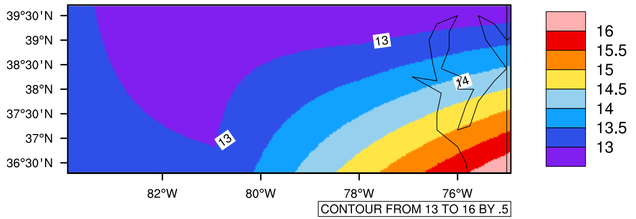
Yearly tas(c) In 2070-2079 GFDL-ESM2M RCP85 - Virginia
