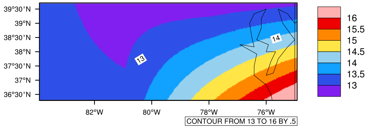
Yearly tas(c) In 2080-2089 GFDL-ESM2M RCP85 - Virginia
