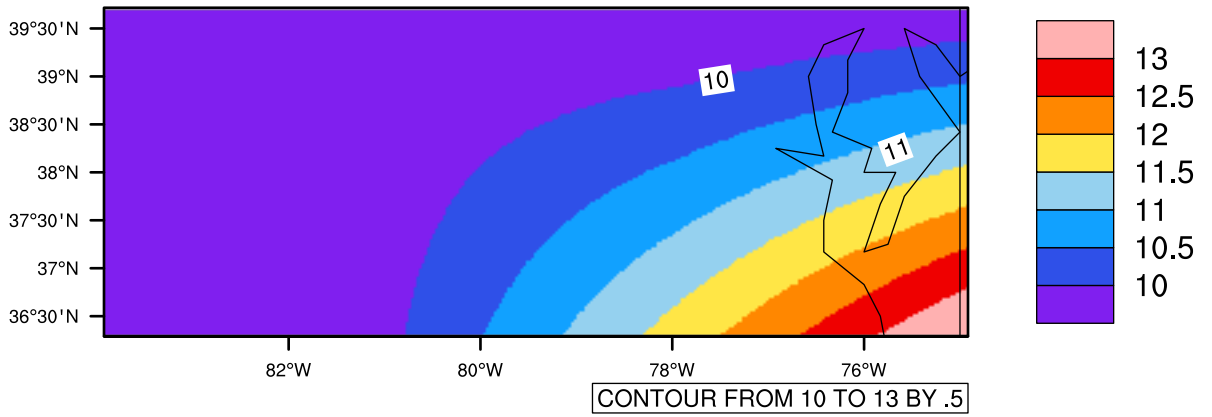
Yearly tas(c) In 1975-2005 GFDL-ESM2M historical - Virginia
