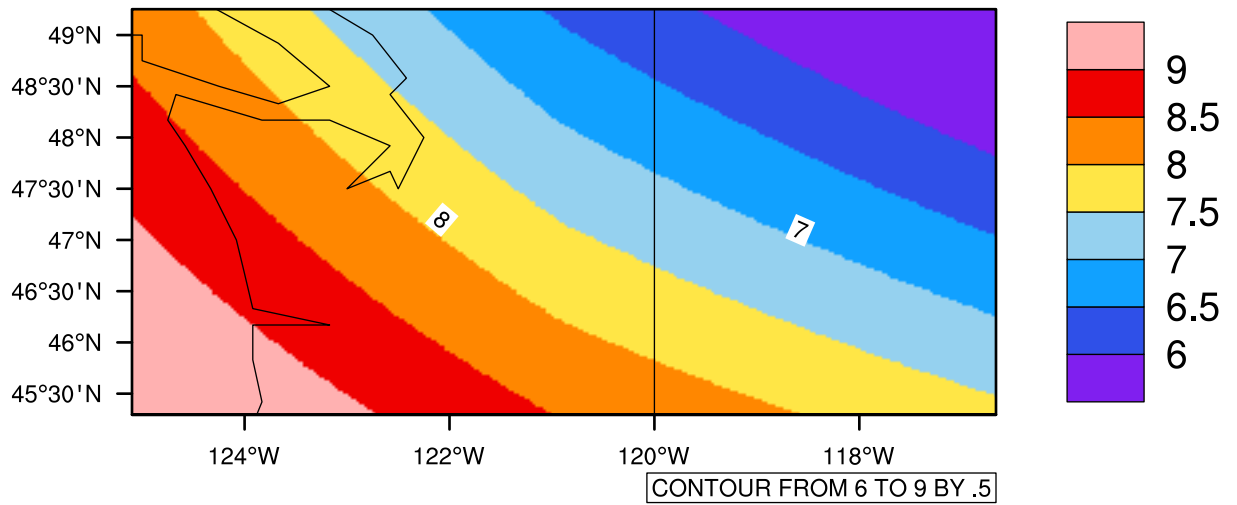
Yearly tas(c) In 2040-2049 GFDL-ESM2M RCP45 - Washington
