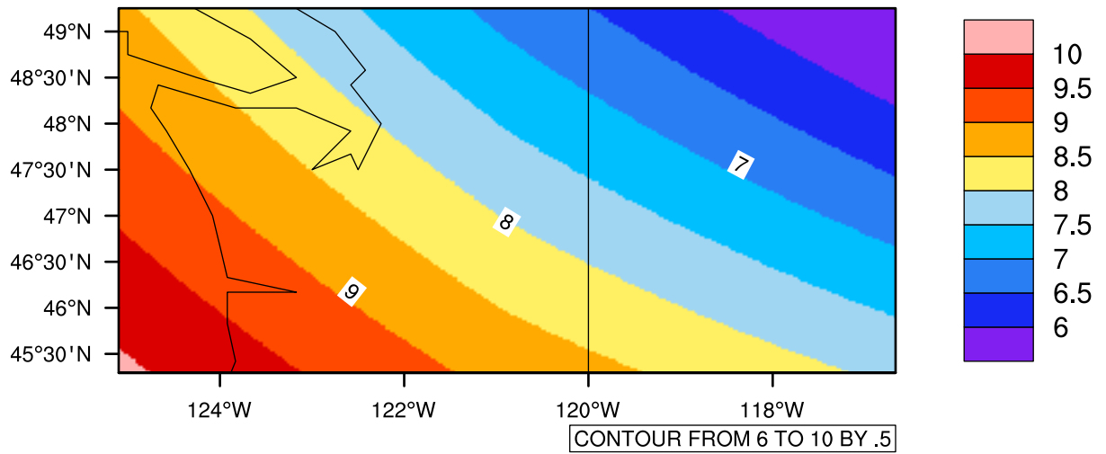
Yearly tas(c) In 2050-2059 GFDL-ESM2M RCP45 - Washington
