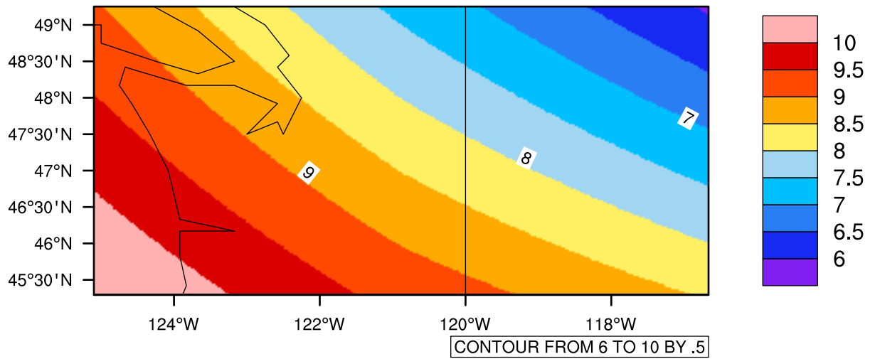
Yearly tas(c) In 2060-2069 GFDL-ESM2M RCP45 - Washington
