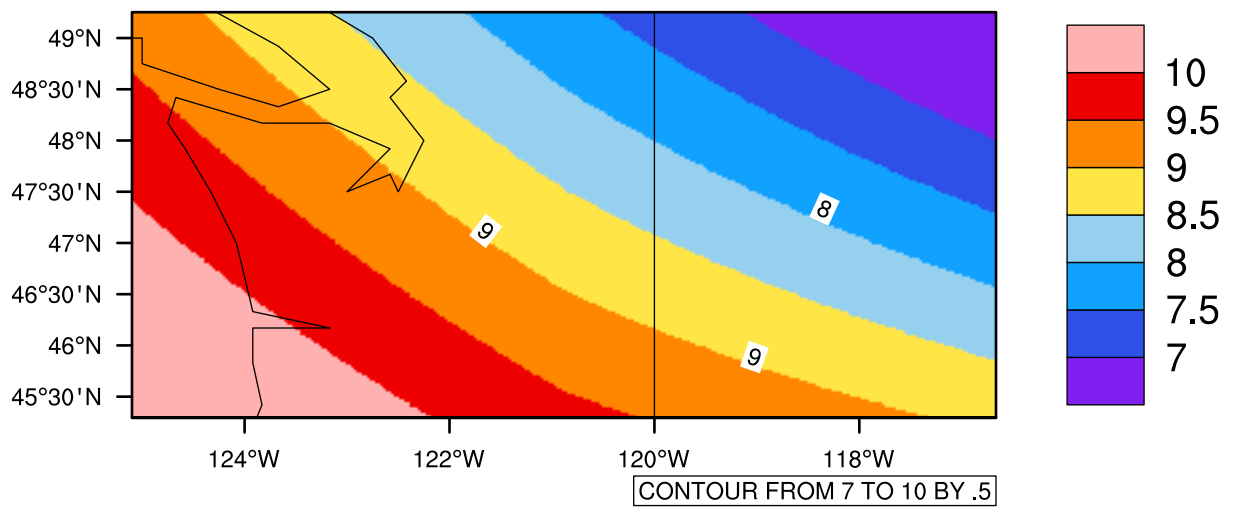
Yearly tas(c) In 2070-2079 GFDL-ESM2M RCP45 - Washington
