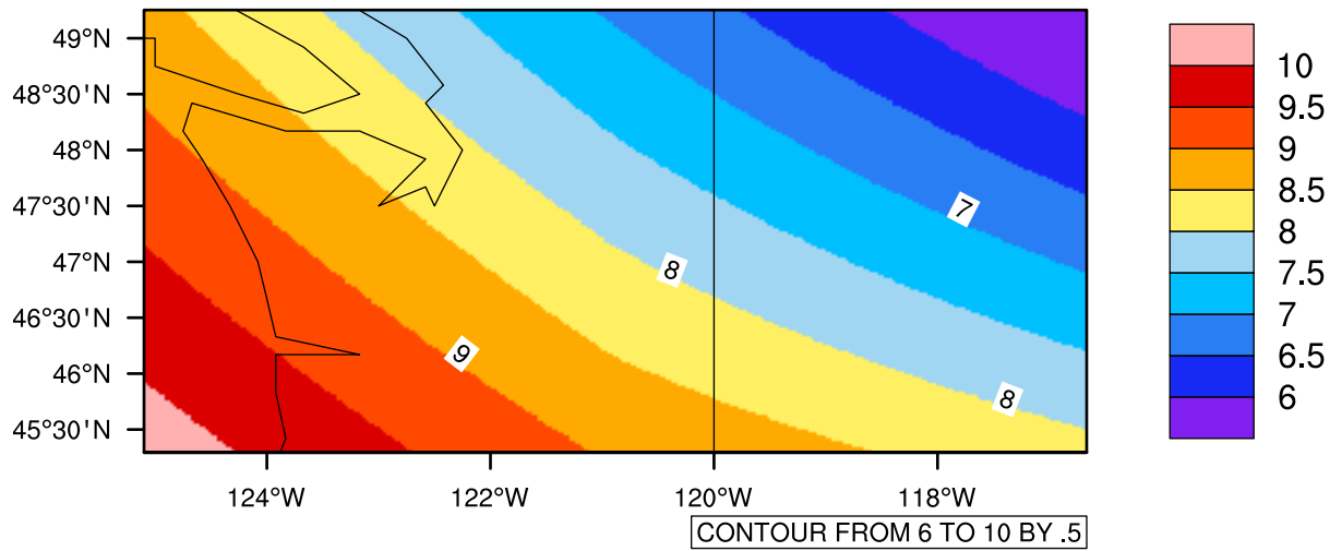
Yearly tas(c) In 2080-2089 GFDL-ESM2M RCP45 - Washington
