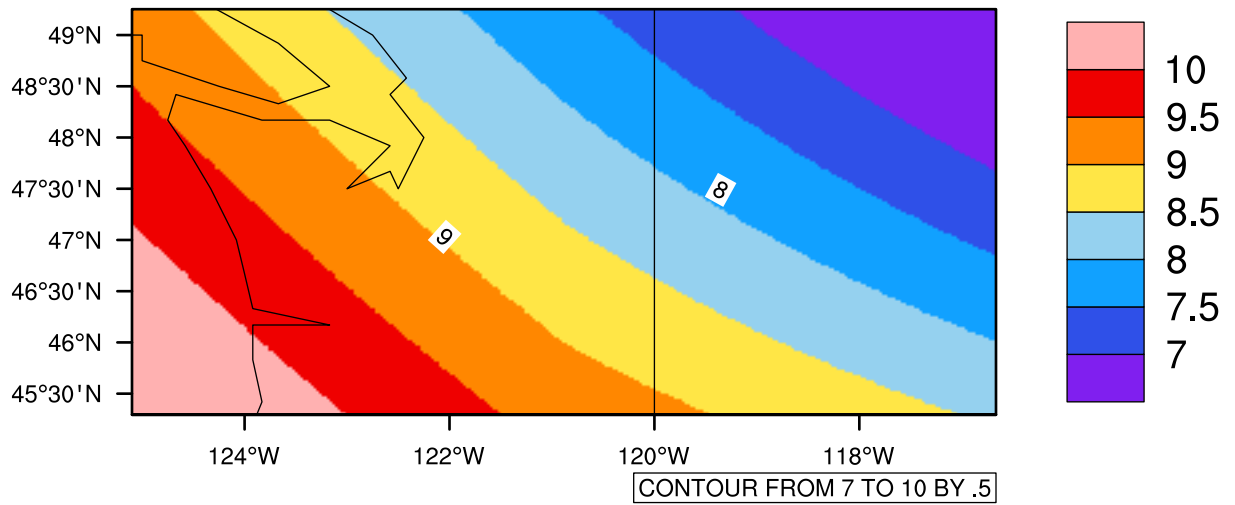
Yearly tas(c) In 2090-2099 GFDL-ESM2M RCP45 - Washington
