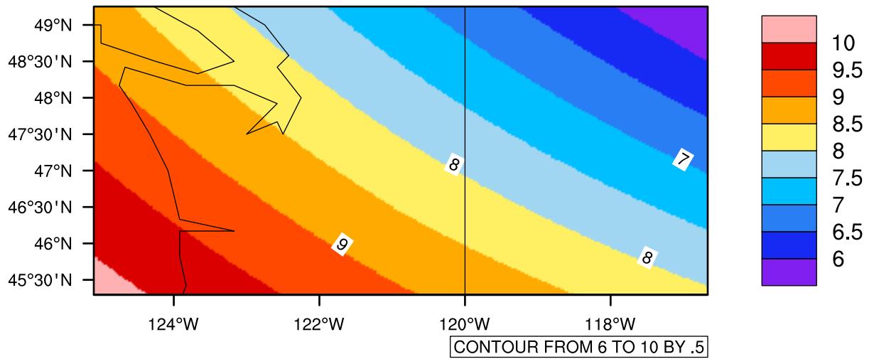
Yearly tas(c) In 2030-2039 GFDL-ESM2M RCP85 - Washington
