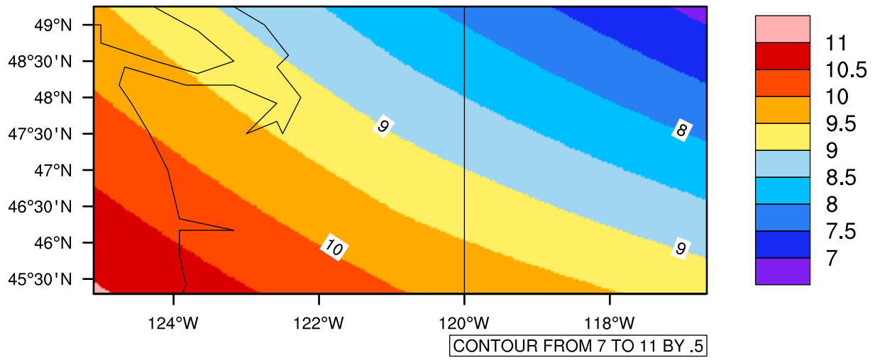
Yearly tas(c) In 2050-2059 GFDL-ESM2M RCP85 - Washington
