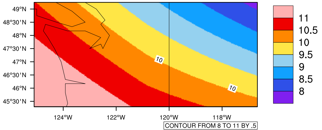
Yearly tas(c) In 2080-2089 GFDL-ESM2M RCP85 - Washington
