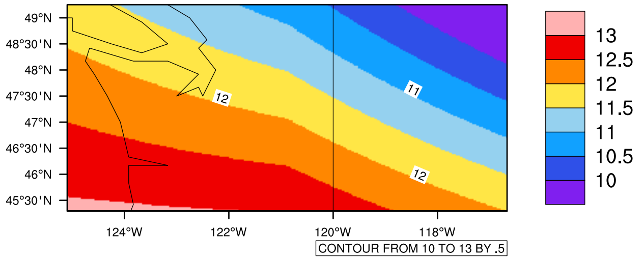
Yearly tasmax(c) In 2030-2039 GFDL-ESM2M RCP85 - Washington
