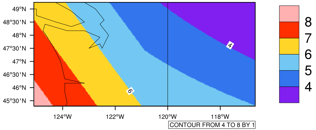
Yearly tasmin(c) In 2040-2049 GFDL-ESM2M RCP85 - Washington
