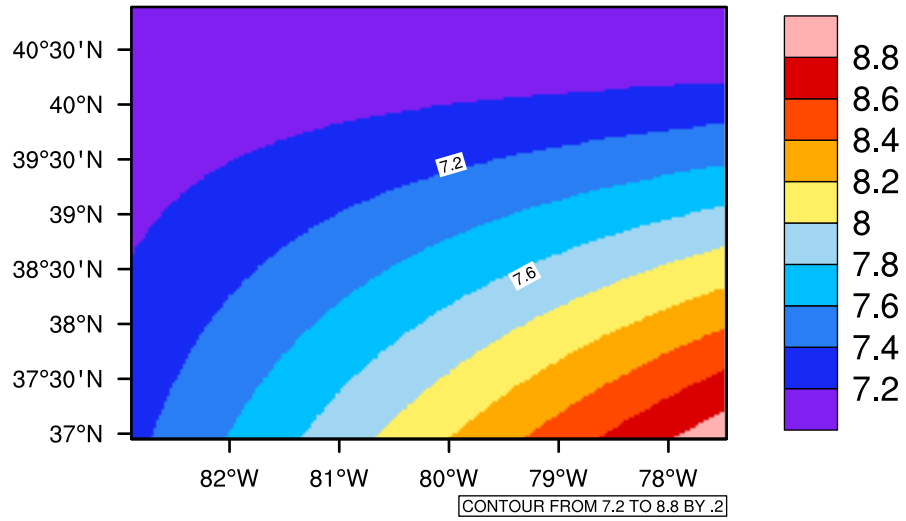
Yearly tasmin(c) In 2020-2029 GFDL-ESM2M RCP45 - West Virginia
