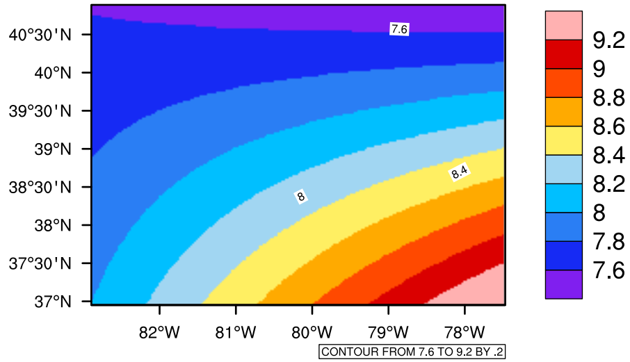
Yearly tasmin(c) In 2040-2049 GFDL-ESM2M RCP45 - West Virginia
