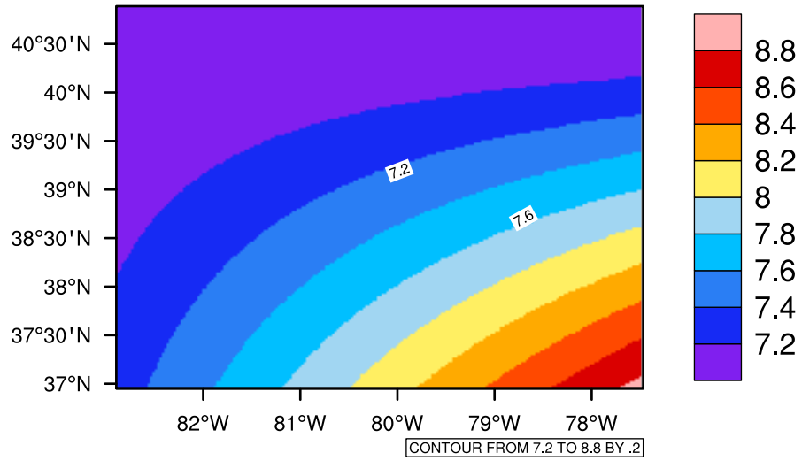
Yearly tasmin(c) In 2020-2029 GFDL-ESM2M RCP85 - West Virginia
