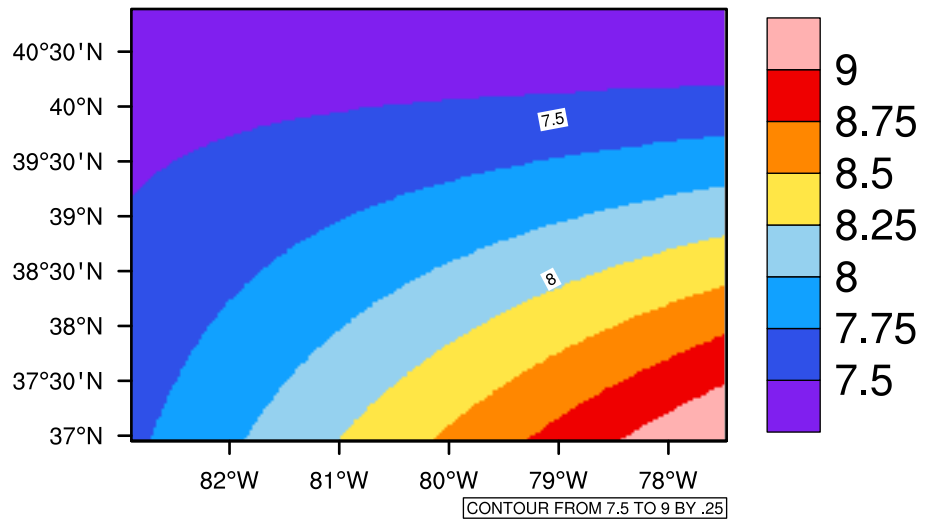
Yearly tasmin(c) In 2040-2049 GFDL-ESM2M RCP85 - West Virginia
