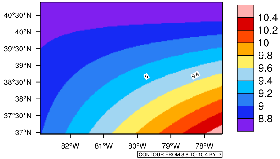
Yearly tasmin(c) In 2060-2069 GFDL-ESM2M RCP85 - West Virginia
