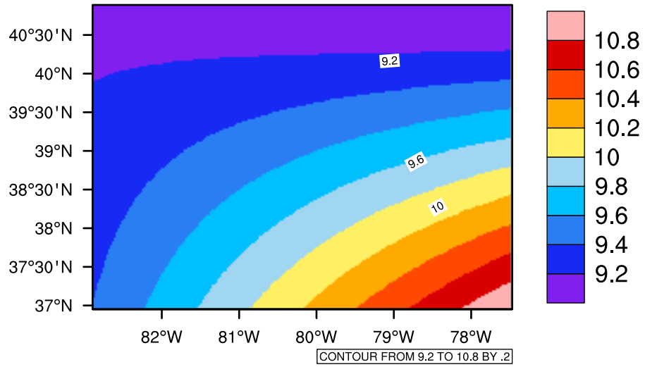
Yearly tasmin(c) In 2070-2079 GFDL-ESM2M RCP85 - West Virginia
