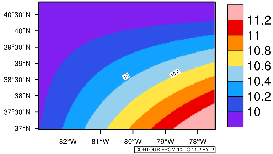
Yearly tasmin(c) In 2090-2099 GFDL-ESM2M RCP85 - West Virginia
