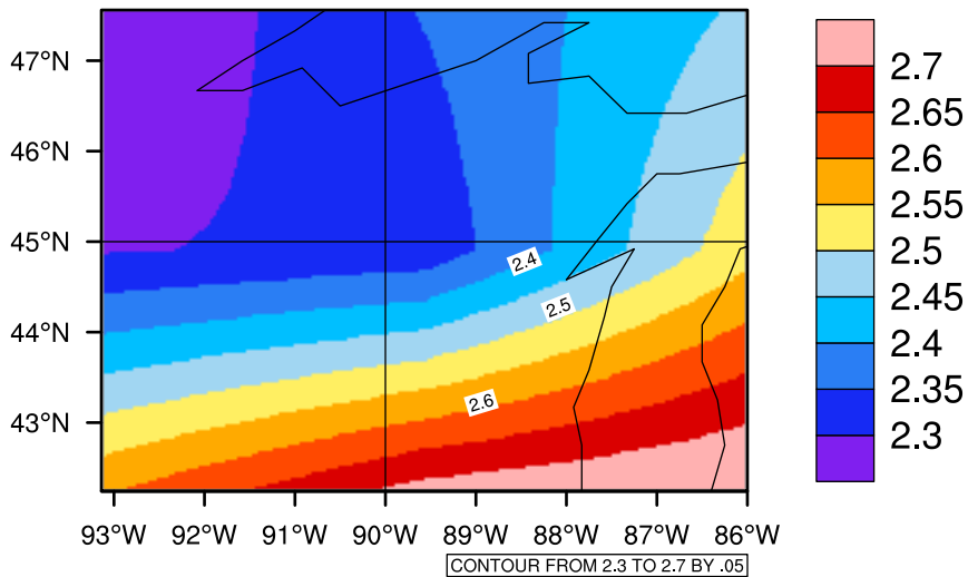
Yearly pr (mm/day) In 2020-2029 GFDL-ESM2M RCP45 - Wisconsin
