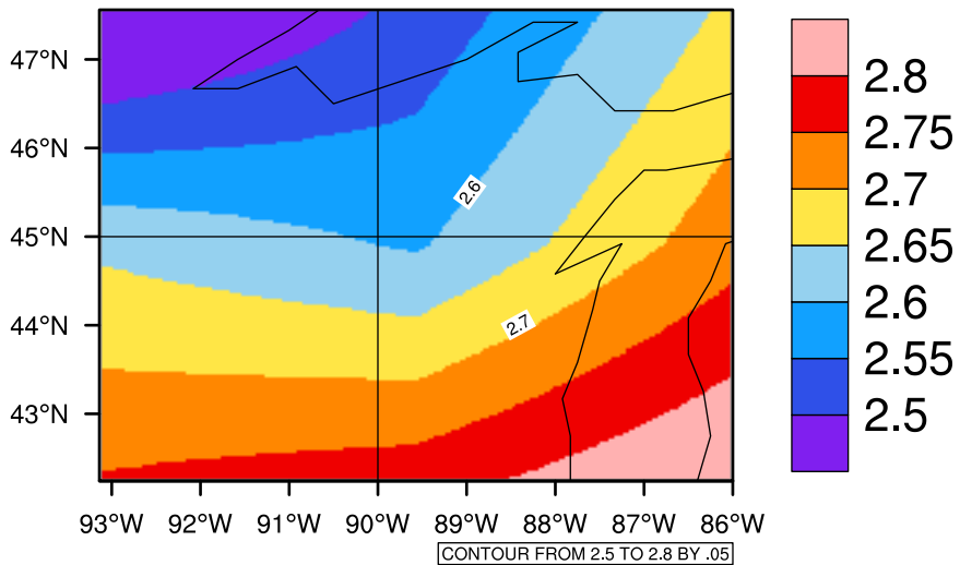
Yearly pr (mm/day) In 2060-2069 GFDL-ESM2M RCP45 - Wisconsin
