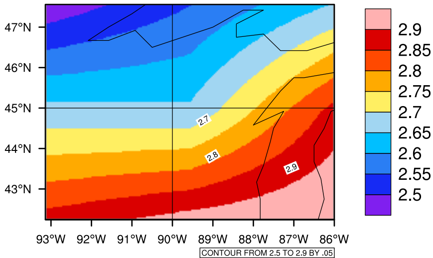
Yearly pr (mm/day) In 2070-2079 GFDL-ESM2M RCP45 - Wisconsin
