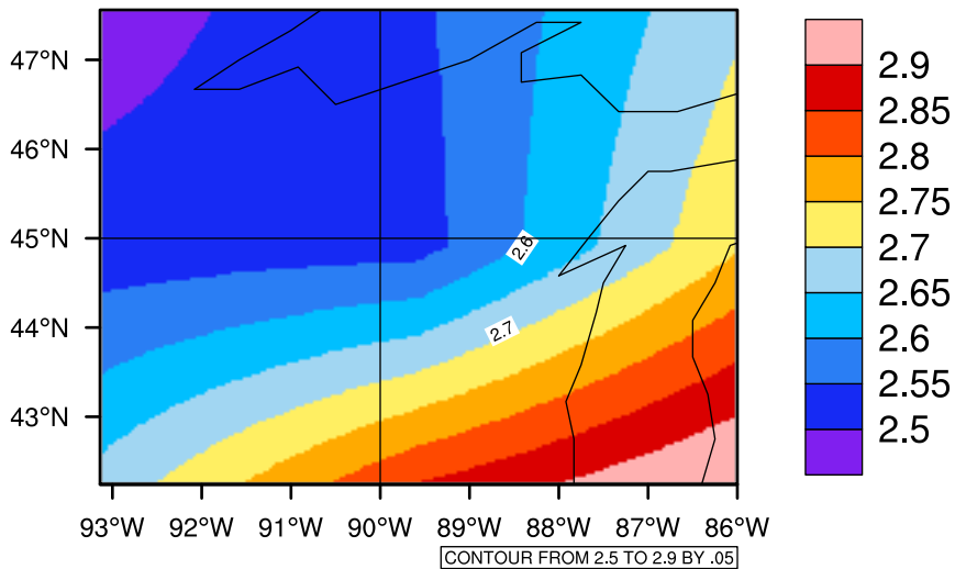
Yearly pr (mm/day) In 2080-2089 GFDL-ESM2M RCP45 - Wisconsin
