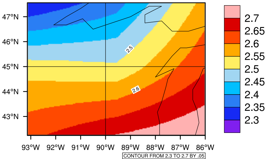
Yearly pr (mm/day) In 2040-2049 GFDL-ESM2M RCP85 - Wisconsin
