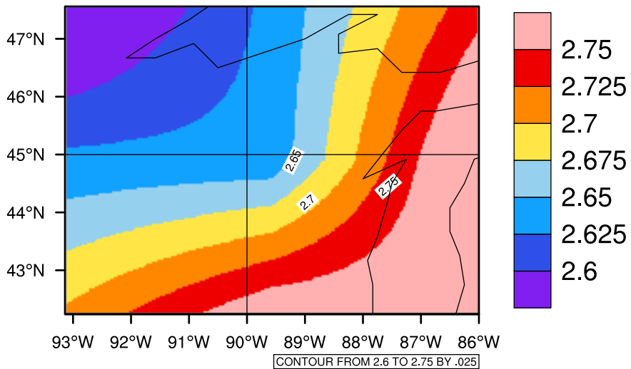
Yearly pr (mm/day) In 2070-2079 GFDL-ESM2M RCP85 - Wisconsin
