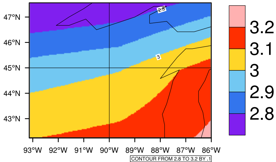
Yearly pr (mm/day) In 2080-2089 GFDL-ESM2M RCP85 - Wisconsin
