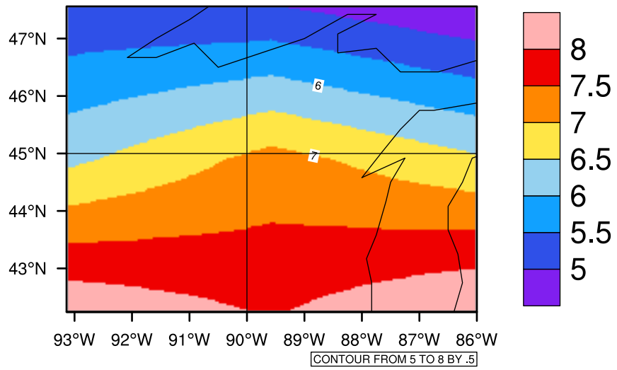
Yearly tas(c) In 2020-2029 GFDL-ESM2M RCP85 - Wisconsin
