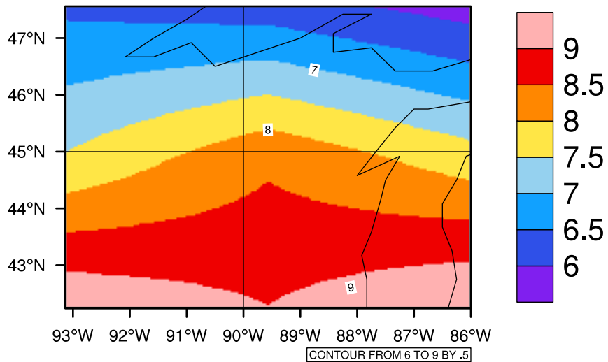
Yearly tas(c) In 2030-2039 GFDL-ESM2M RCP85 - Wisconsin
