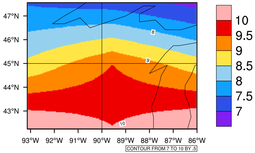
Yearly tas(c) In 2050-2059 GFDL-ESM2M RCP85 - Wisconsin
