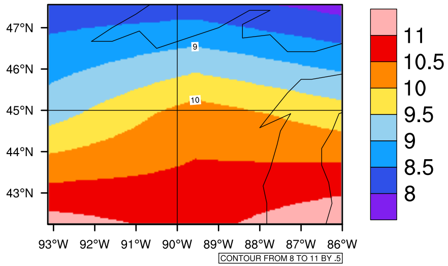
Yearly tas(c) In 2080-2089 GFDL-ESM2M RCP85 - Wisconsin
