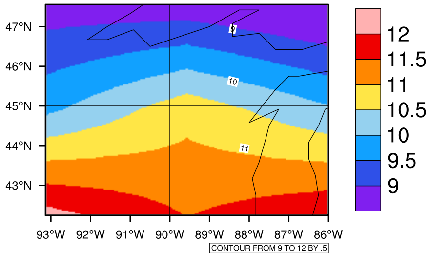
Yearly tas(c) In 2090-2099 GFDL-ESM2M RCP85 - Wisconsin
